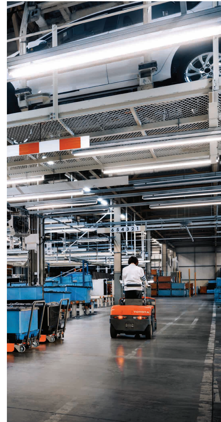
S-series' low step-in height makes getting on and off easy. The Operator Presence System (left-hand pedal) ensures that the truck cannot be driven unless the operator is standing in the correct position.
